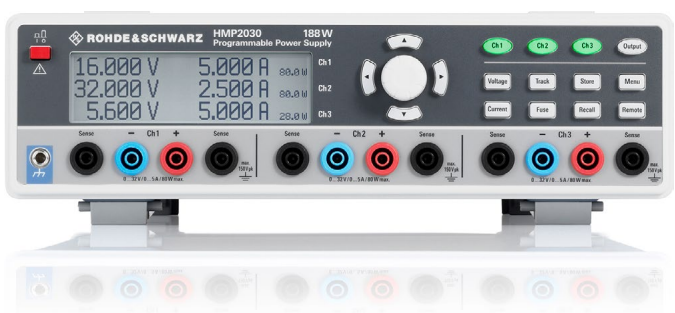
R&S®HMP2030 three-channel instrument.
