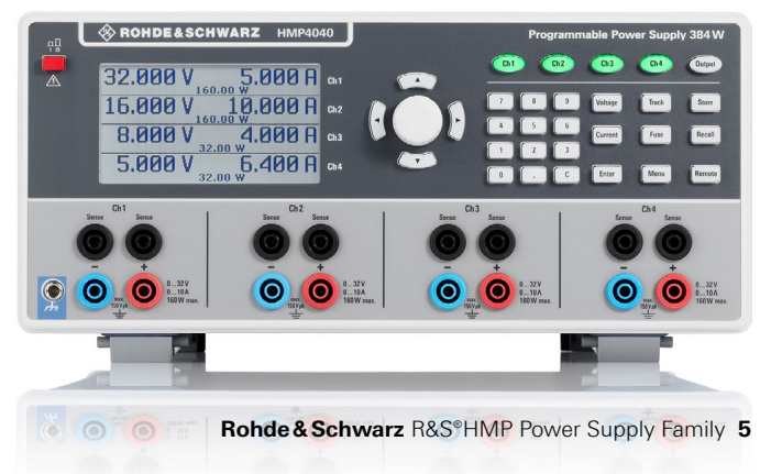
R&S ® HMP4040 four-channel instrument.
